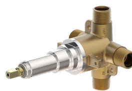
Triple Outlet Diverter Valve Body 3DIVBODYSRT SPEC: TUB-TRM27K
