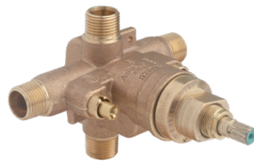
Temptrol Tub/Shower Valve Body with Stops 262XBODY SPEC: TUB-TRM18SY
